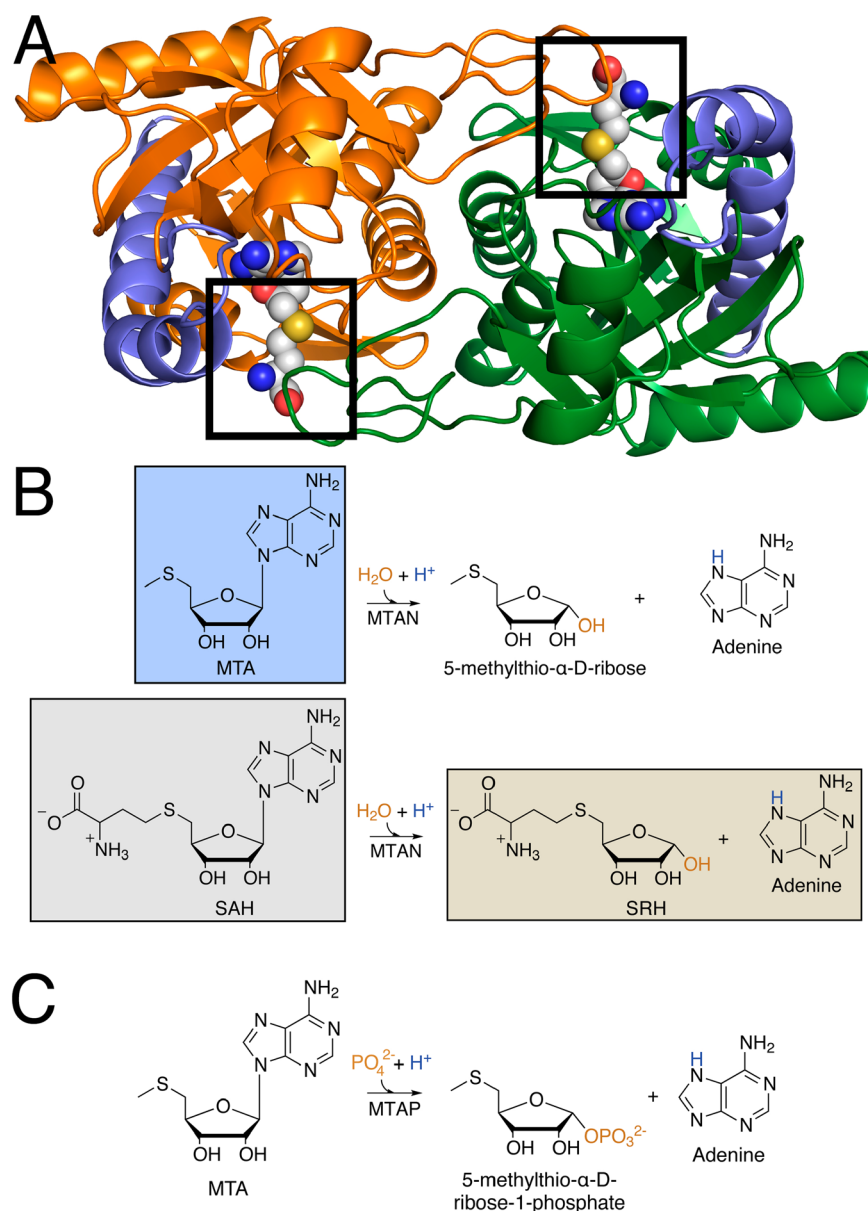
Figure 2. Shared active site in the HpMTAN homodimer and the enzyme mechanism. (A) The closed form of the HpMTAN -D198N active site is shown with SAH (spheres colored by CPK) bound. The cartoons (orange and green) represent the HpMTAN homodimer. The position of helix \alpha 6 is indicated for each monomer in light blue. The boxed regions indicate the location of the 5'-alkylthio binding subsite that interacts with the homocysteine moiety of SAH. (B) Reactions proposed for the two most commonly studied MTAN substrates. The ligands for each of the determined structures are highlighted in boxes. The substrates are colored black; the nucleophile is colored orange, and the MTAN-derived proton is colored blue. (C) Proposed reaction for the human MTAP enzyme. The coloring of the components is the same as in panel B.
